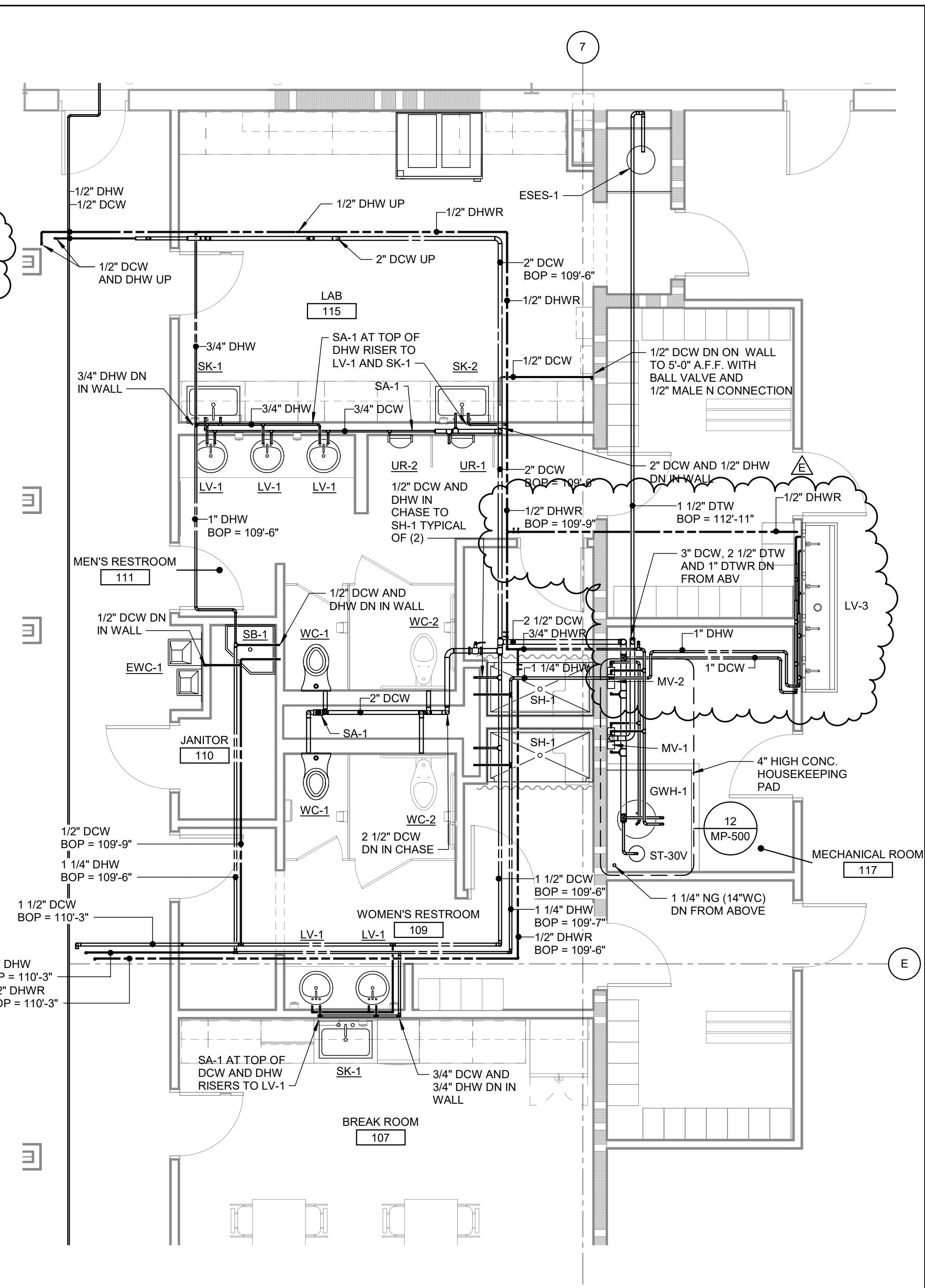
3 ENLARGED FIRST FLOOR OFFICE TOILET WATER PLAN MH-300 SCALE: 1/4" = 1'-0" FFE= 100'-0" Scale: 1/4" = 1'-0"
