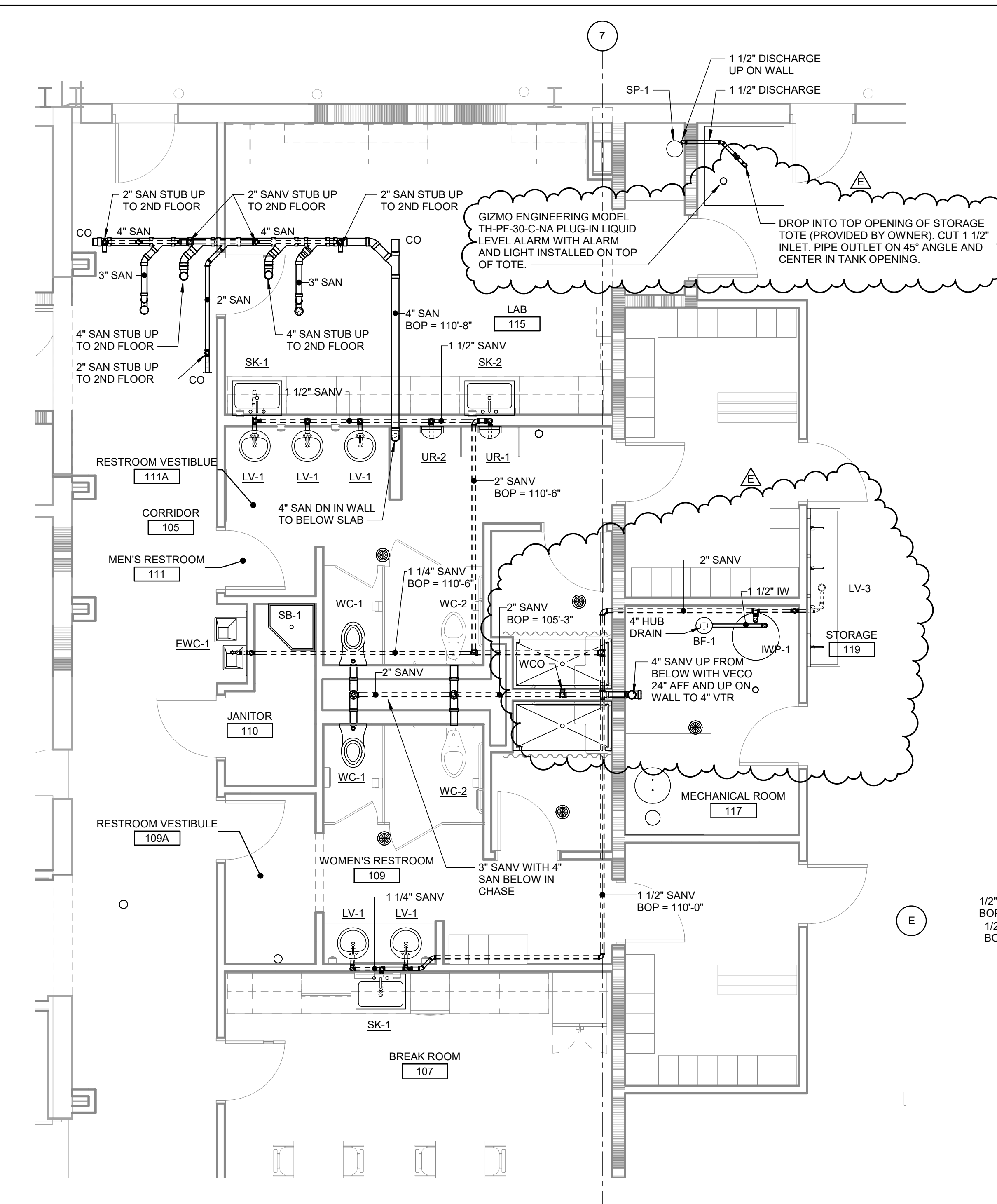
2 ENLARGED FIRST FLOOR OFFICE TOILET SAN / SANV PLAN MH-300 SCALE: 1/4" = 1'-0" FFE= 100'-0" Scale: 1/4" = 1'-0"
