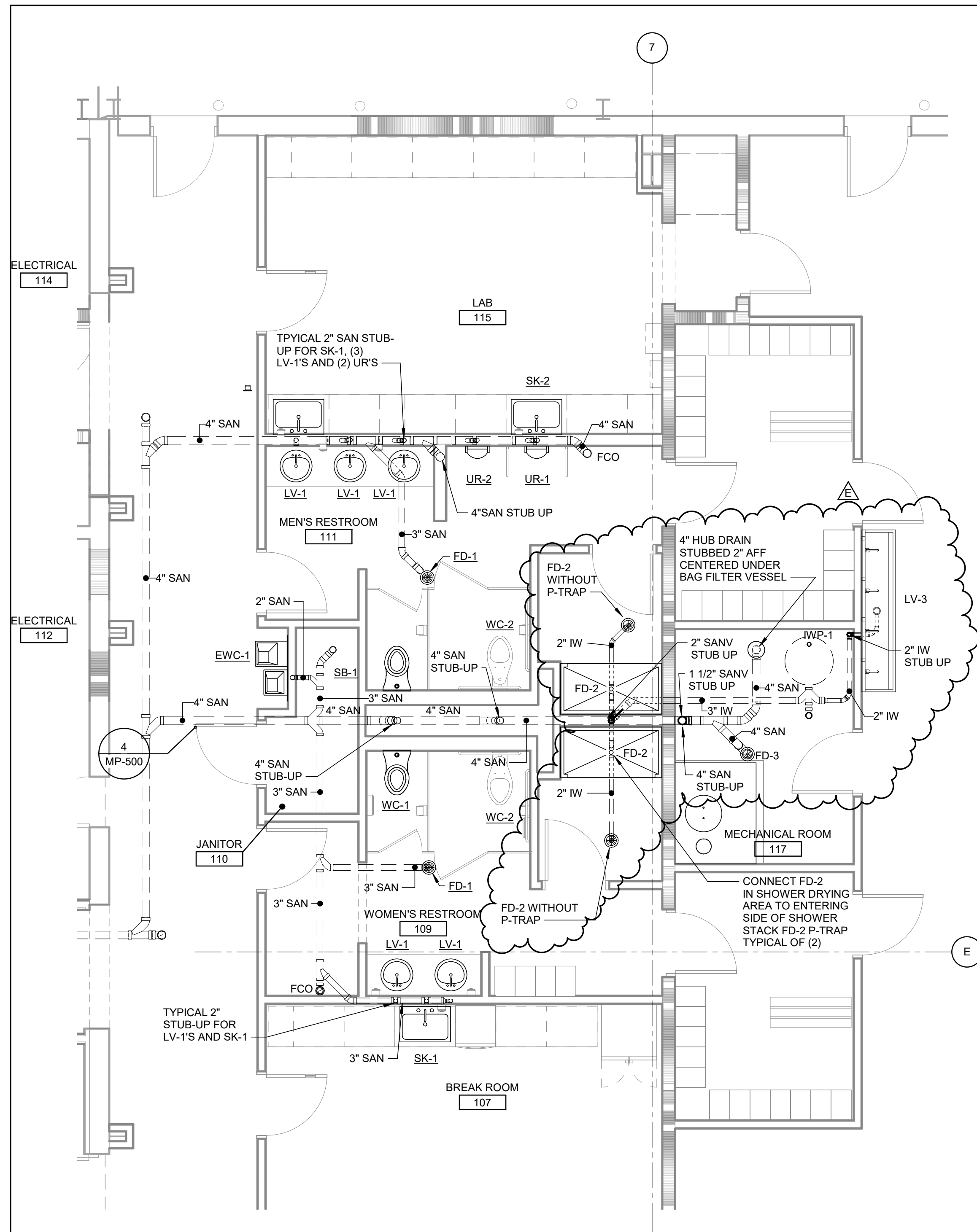
1 ENLARGED FIRST FLOOR OFFICE TOILET UNDERGROUND SAN PLAN MH-300 SCALE: 1/4" = 1'-0" FFE= 100'-0" Scale: 1/4" = 1'-0"
