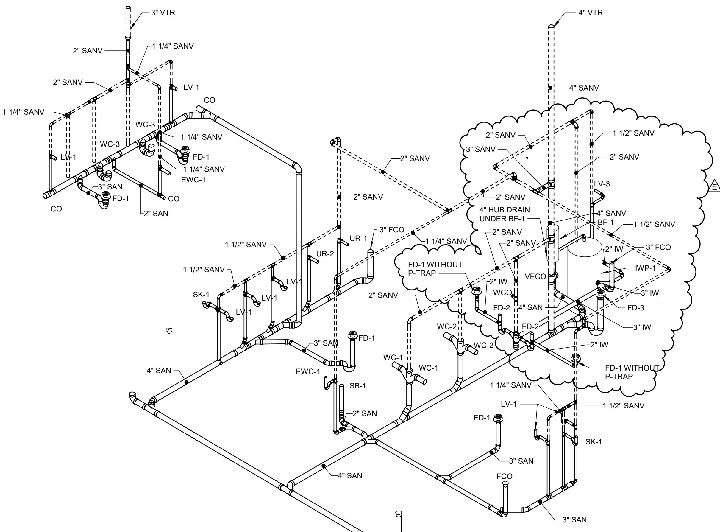
4 FIRST FLOOR OFFICE TOILET SAN / SANV ISOMETRIC SCALE: NOT TO SCALE
